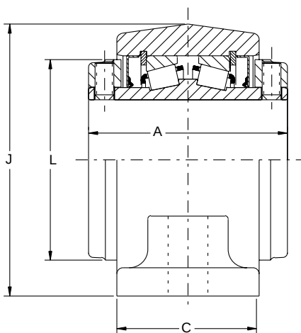
1-3/16" THRU 3" CONSTRUCTION
