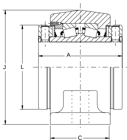
3-3/16" THRU 3-1/2" CONSTRUCTION
